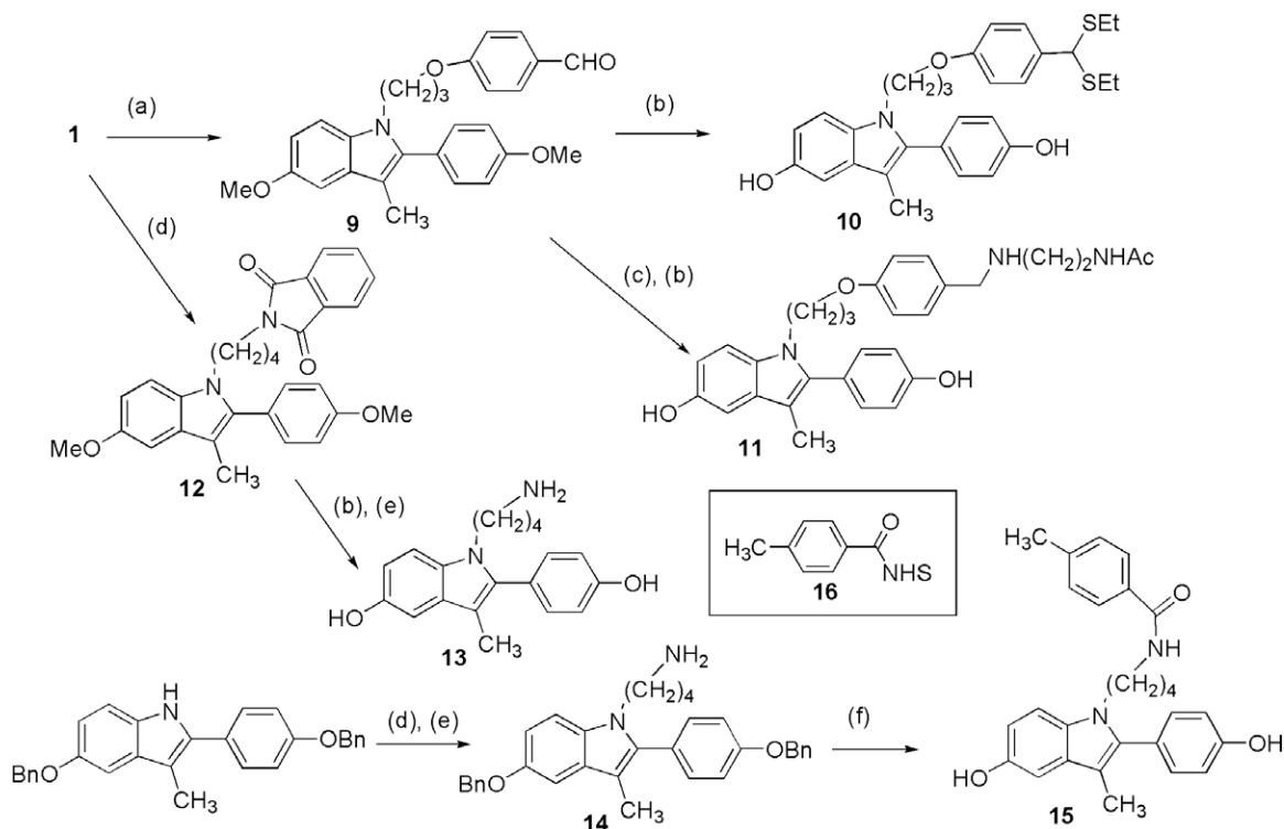
Scheme 2. Reagents and conditions: (a) NaH, 4-(3-iodopropoxy)benzaldehyde, DMF, 79%; (b) EtSH, AlCl 3 , rt, 89%-quant; (c) i-NH 2 (CH 2 ) 2 NHAc, MeOH, 65 °C; ii-NaBH 4 , MeOH; (d) NaH, 4-iodobutylphthalimide, rt, 62–83%; (e) H 2 NNH 2 , CH 2 Cl 2 /CHCl 3 , MeOH, rt, quant; (f) i- 16 , CH 2 Cl 2 , quant; ii-Pd/C, MeOH, quant.
