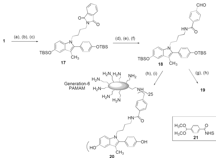
Scheme 3. Reagents and conditions: (a) NaH, 4-iodobutylphthalimide, DMF, 0 °C to rt, 83%; (b) EtSH, AlCl 3 , rt, 85%; (c) TBDMSCl, imidazole, DMF, 91%; (d) H 2 NNH 2 , CH 2 Cl 2 , MeOH, rt, 80%; (e) 21 , CH 2 Cl 2 , THF, rt, 80%; (f) H + , acetone, rt, 72%; (g) i-NH 2 CH 2 CH 2 NHAc, CH 2 Cl 2 , ii-NaBH 4 ; (h) 1N HCl/MeOH, rt, quant; (i) i-G-6 PAMAM, MeOH, rt; ii-NaBH 4 , quant.
